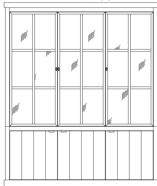
VITRINE 3Y - 3 DOORS METAL 1840 x 480 x 2190(H)
