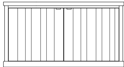
BUFET 2 DOORS + 1 DRAWERS 1634 x 480 x 885(H)
