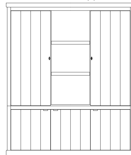
VITRINE 3oW - 2 DOORS WOOD + MIDDLE OPEN (LEFT AND RIGHT DOOR WOOD) 1840 x 480 x 2190(H)
