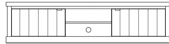
TV CHEST 2 DOORS 2000 x 480 x 500(H)
