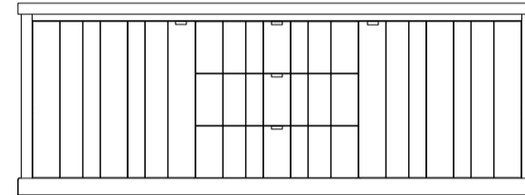
BUFET 2 DOORS + 3 DRAWERS 2380 x 480 x 885(H)
